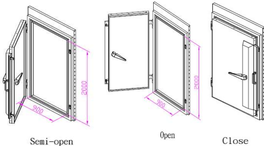
Shielding door size:(W)0.9m*(H)2 m
